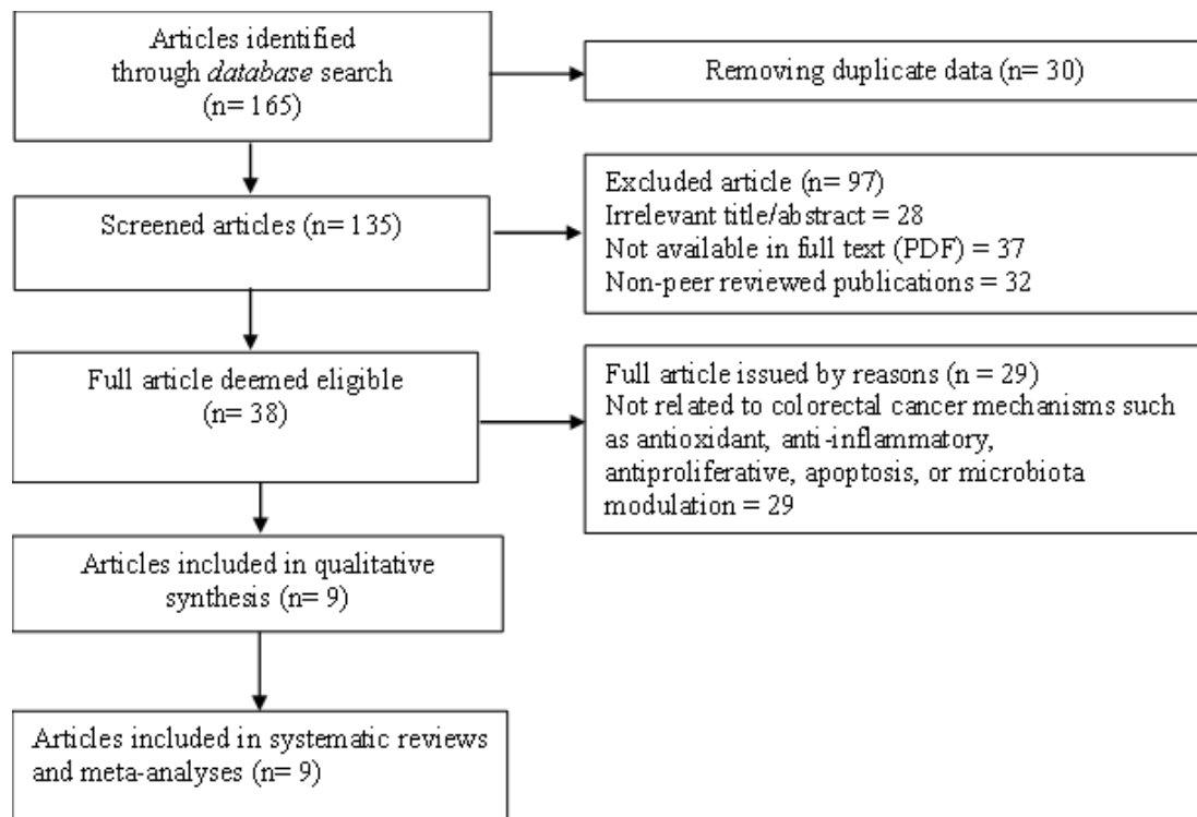
Figure 1. Prisma Flowchart
